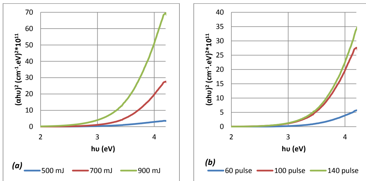
Fig.(6): Shows the energy band gap of the UV-Vis measurement for different (a) Laser energies and (b) Number of laser pulses.
