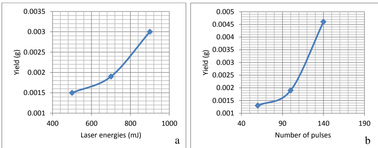
Fig.(3): Yield measurements of ZnO nano particles suspensions in ethanol solvent at two parameters (a) laser energies and (b) laser pulses.
