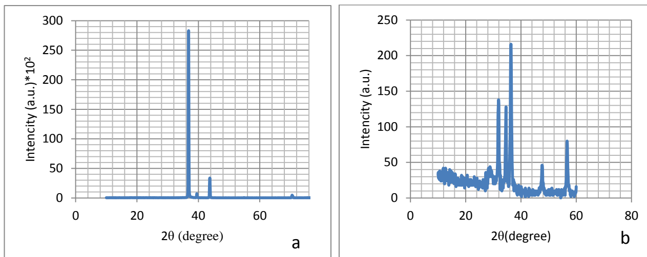
Fig.(2): XRD spectra of (a) Zn target as a pellet and (b) ZnO target as a nano particles thin film prepared by electrophoretic deposition (EPD).
