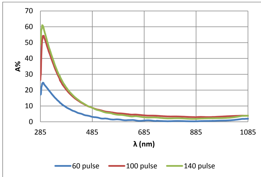
Fig.(5): Shows the absorption of the UV-Vis measurement for different number of laser pulses.
