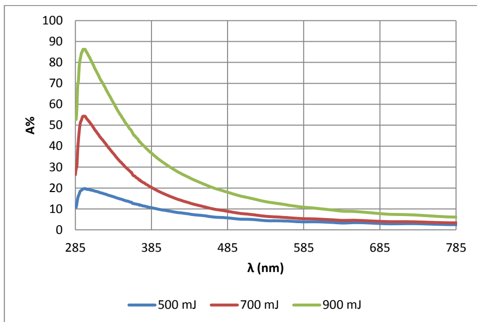
Fig.(4): Shows the absorption of the UV-Vis measurement for different laser energies.
