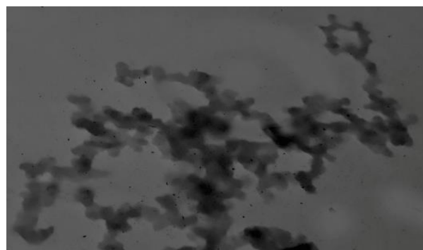
Fig.(7): Shows the TEM morphology of prepared nano particles of ZnO nano particles formed by ablation of Zn target immersed in ethanol of laser energy of 500 mJ and laser pulse of 100 pulses.
