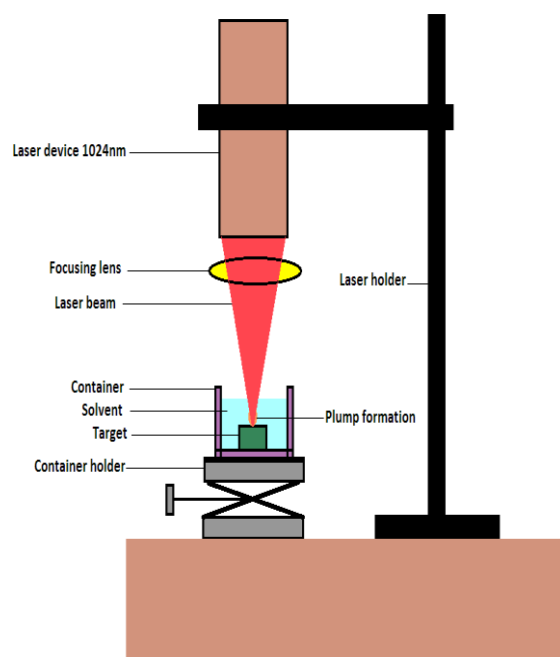
Fig.(1): Experimental setup for liquid phase laser ablation system.
